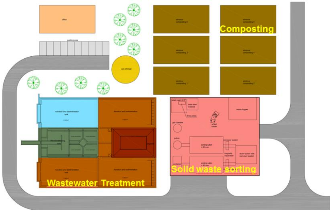
Figure 2. Example for a DUPLEX plant (capacity 20,000 PE).
